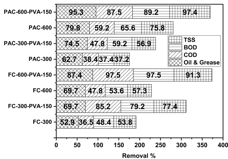
Figure 9. Comparison of eight experiments along with Oil & Grease, COD, BOD and TSS removal percentages
