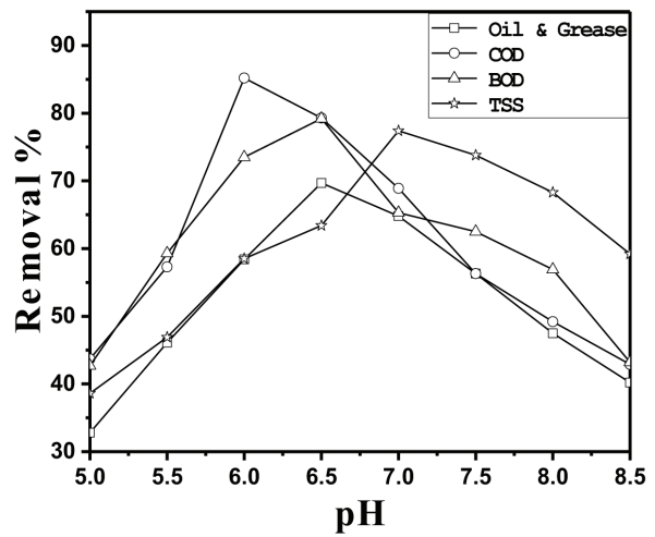
Figure 2. Effect of pH on the removal capacity of Ferric Chloride with 90 mg/300 ml dosing coupled with PVA 45 mg/300 ml
