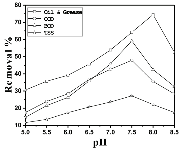
Figure 6. Effect of pH on the removal capacity of PAC with 90 mg/L dosing coupled with 45 mg/300 ml PVA
