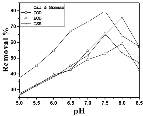
Figure 7. Effect of pH on the removal capacity of PAC with 180 mg/300 ml dosing
