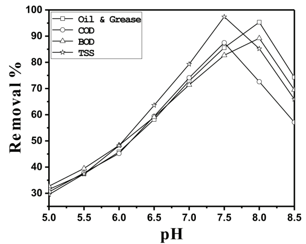
Figure 8. Effect of pH on the removal capacity of PAC with 180 mg/L dosing coupled with 45 mg/L of PVA
