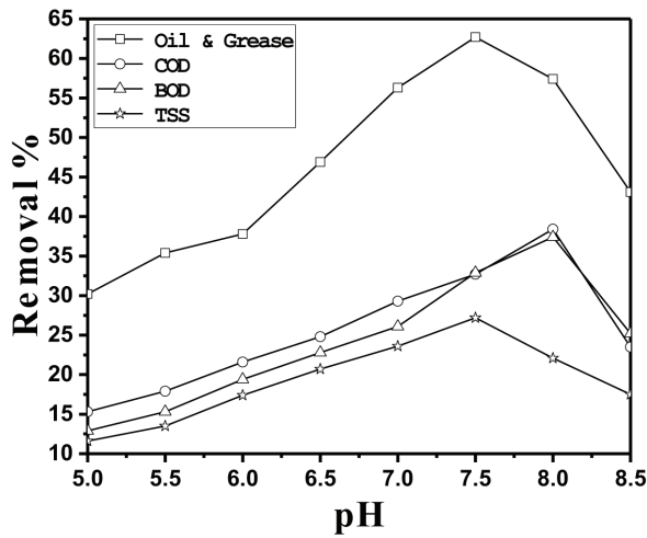
Figure 5. Effect of pH on the removal capacity of PAC with 90 mg/300 ml dosing
