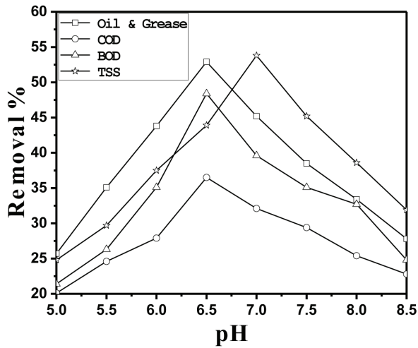
Figure 1. Effect of pH on the removal capacity of Ferric Chloride with 90 mg/300 ml dosing
