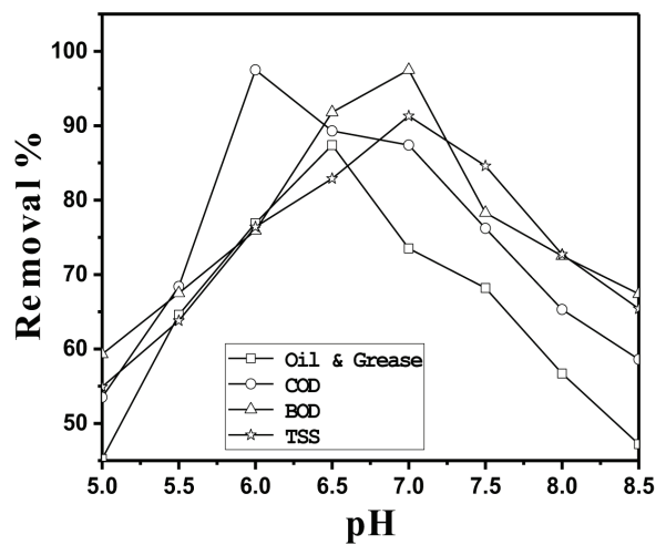
Figure 4. Effect of pH on the removal capacity of Ferric Chloride with 180 mg/L dosing coupled with PVA 45 mg/300 ml
