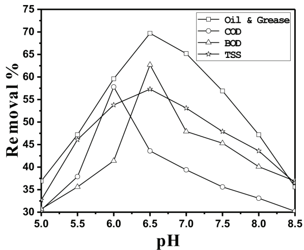
Figure 3. Effect of pH on the removal capacity of Ferric Chloride with 180 mg/300 ml dosing
