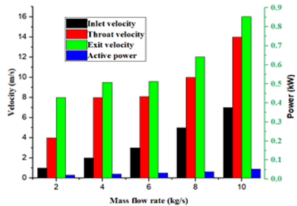
Fig. 10. Distribution of wind velocity over the venturi wind turbine
