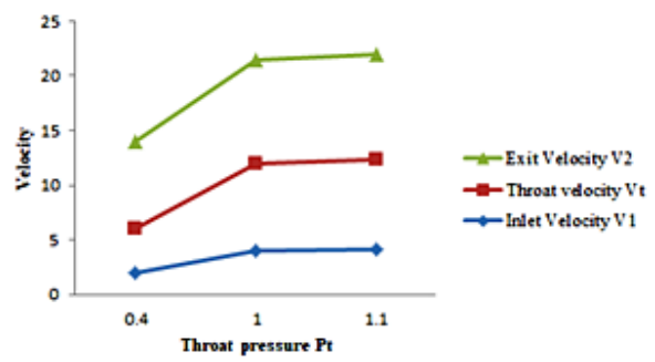
Fig. 8. Throat pressure vs velocities
