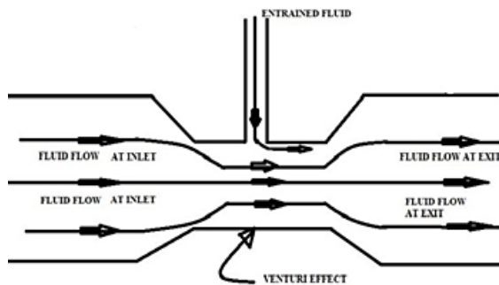
Fig. 2. Working principle of venturi
