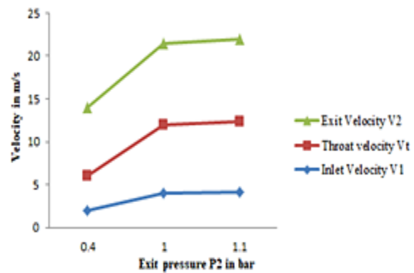
Fig. 9. Exit pressure vs velocity
