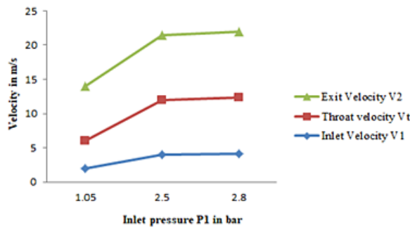
Fig. 7. Pressure distribution vs velocities
