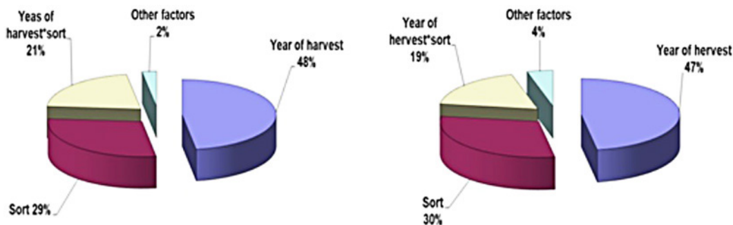
Figure 2. Effect of the factors on seed quality of switch-grass
