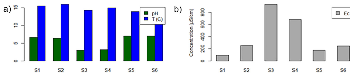
Figure 2. Surface water physicochemical parameters
