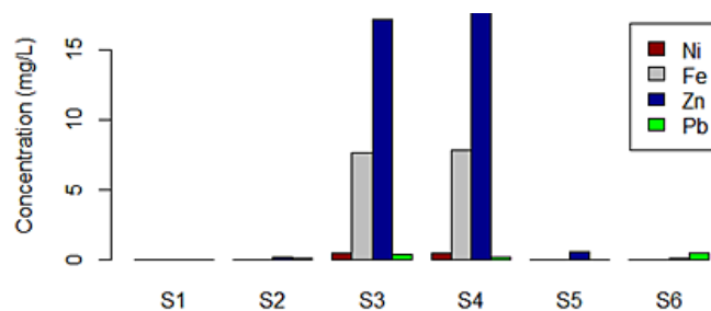
Figure 3. Surface water heavy metals results
