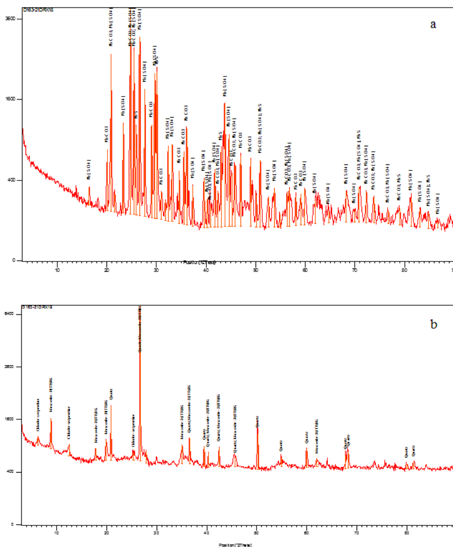
Figure 7. XRD embankments results, (a) Neof ormation minerals and (b) Basement minerals Shales
