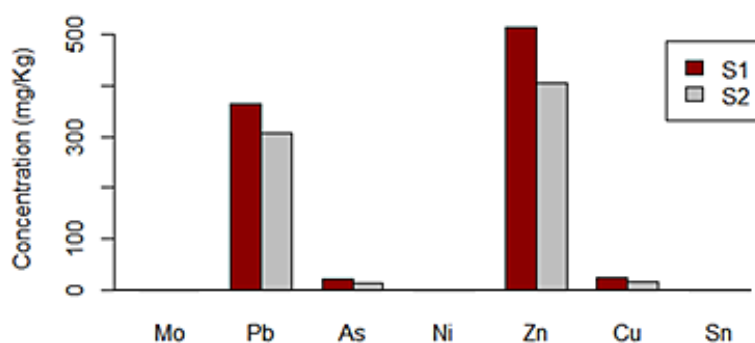
Figure 5. Soil heavy metals results
