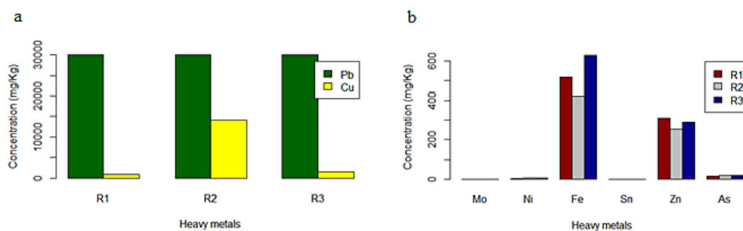
Figure 6. Embankments heavy metals results
