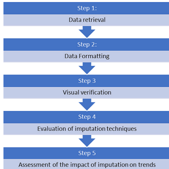
Fig. 3. Working methodology
