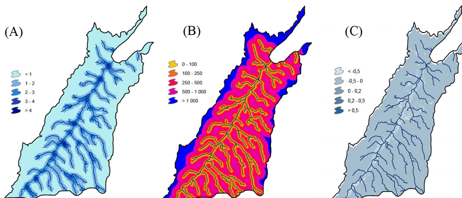
Figure 9. Hydrological factors: (A) drainage density (km/km 2 ) (DD), (B) distance to waterways (m) (DtW) and (C) modified normalized difference water index (MNDWI)
