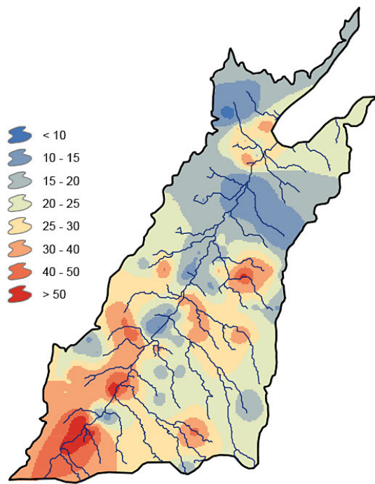
Figure 4. Groundwater depth map (m) (Piezo)
